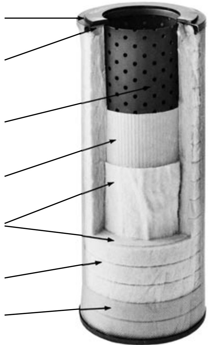
FO-614FG Cutaway
