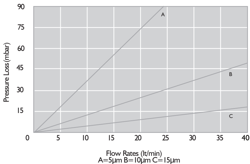
Flow Rates For Water (10" Element)
