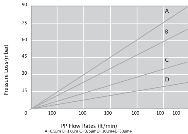
Flow Rates For Water (10" Element)
