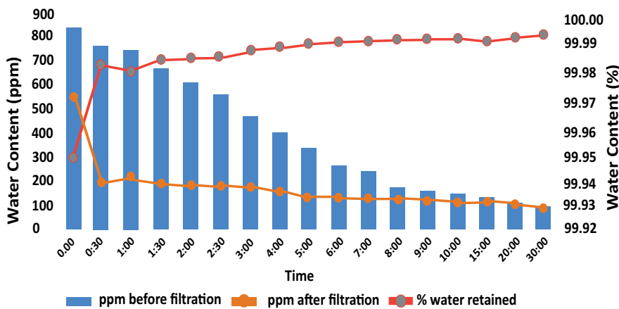
1. Filtasorb2 Water Removal - Diesel Fuel
